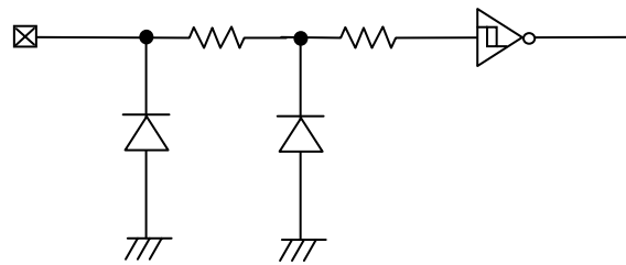
Figure 46. Input Pin Circuit
