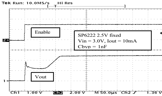
Turn on time, V_{in} = 3.0V , I_{out} = 10mA , CBYP = 1nF
