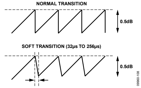
Figure 34. Soft Transition
