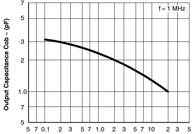
Figure 4. C_{ob} - V_{CB}
