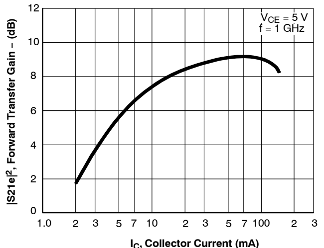
Figure 6. |S_{21e}|^2 - I_C
