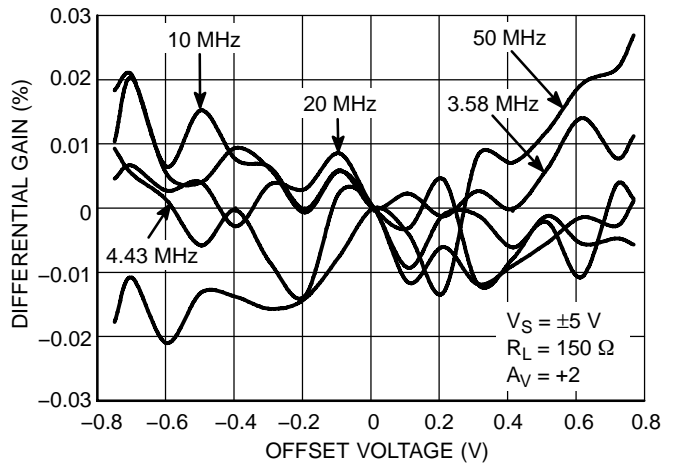
Figure 16. Differential Gain
