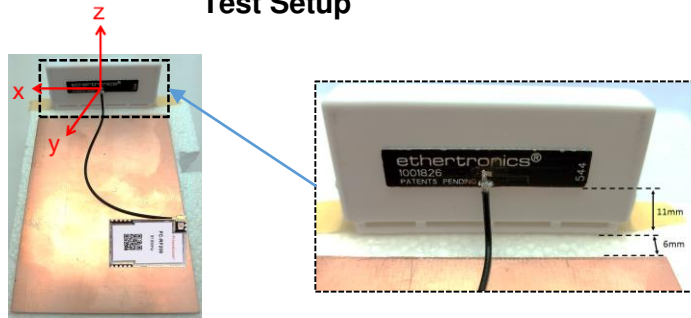
Test Setup
