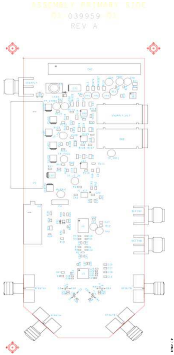
Figure 10. Evaluation Board Silk Screen—Top Side
