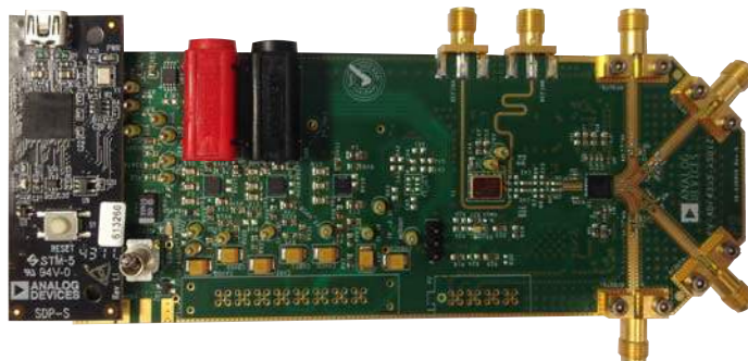
Figure 1. EV-ADF4355-2SD1Z
