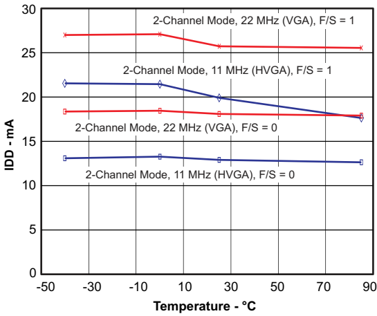
Figure 6-1. Supply Current vs Temperature
