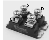
Isolated Baseplate SOT-227
