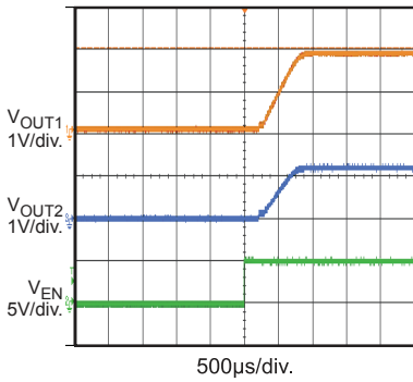
EN On without Load I_{OUT1} = I_{OUT2} = 0A
