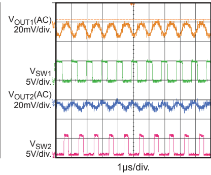
Output Ripple I_{OUT1} = I_{OUT2} = 2A
