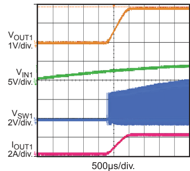
VIN Power On with 2A Load I_{OUT1} = 2A, I_{OUT2} = 0A
