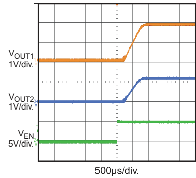
EN On with 2A Load I_{OUT1} = I_{OUT2} = 2A
