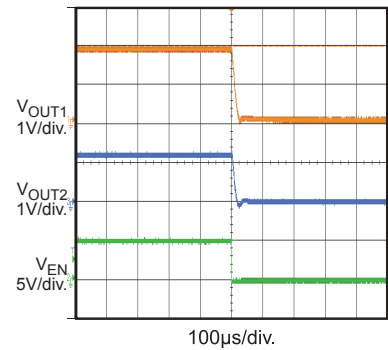
EN Down with 2A Load I_{OUT1} = I_{OUT2} = 2A
