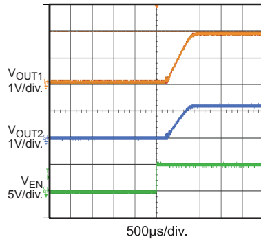
EN On with 1A Load I_{OUT1} = I_{OUT2} = 1A
