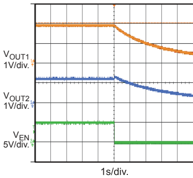
EN Down without Load I_{OUT1} = I_{OUT2} = 0A
