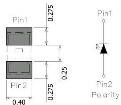
Figure 1. IN-S21AT2G Solder Pattern
