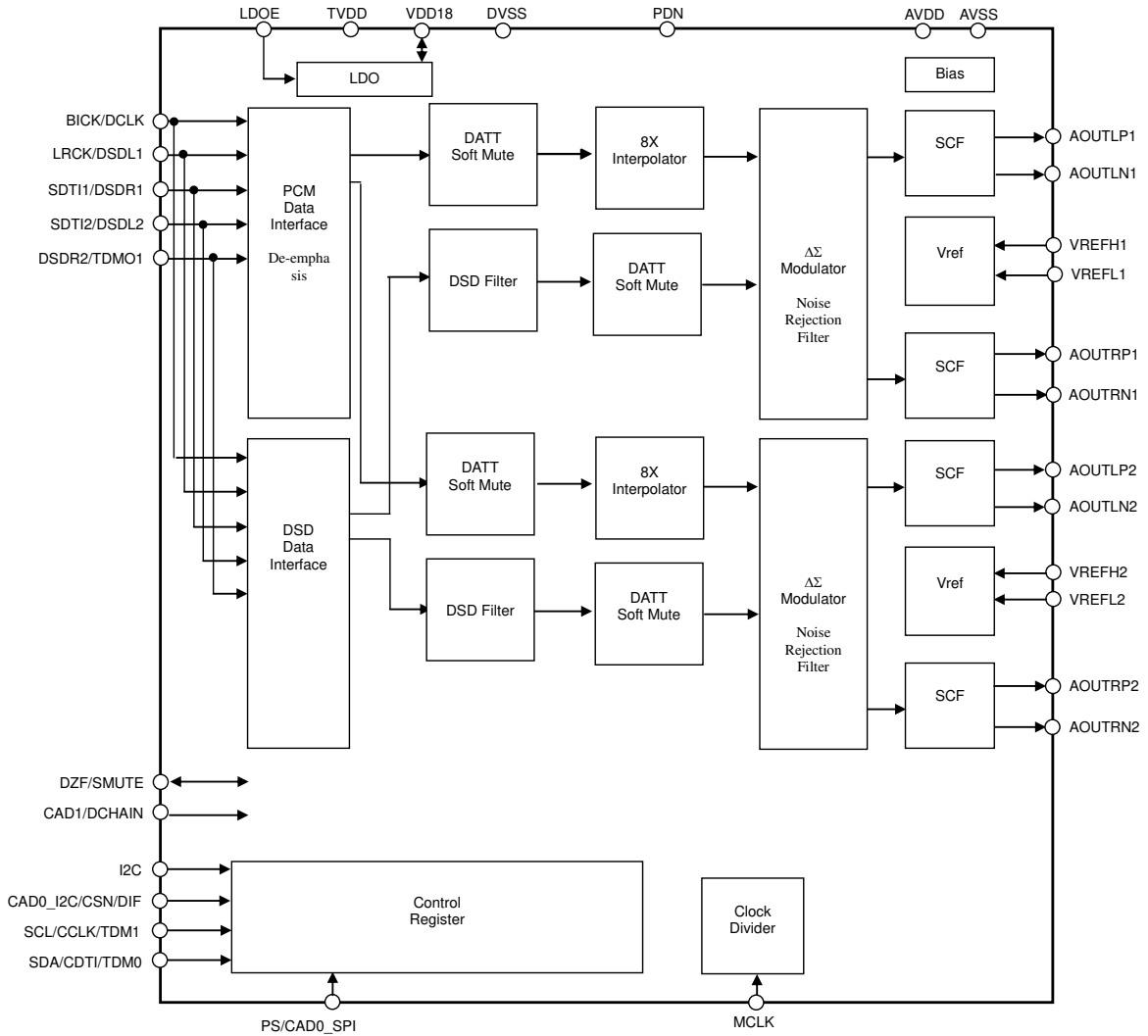
Figure 1. Block Diagram
