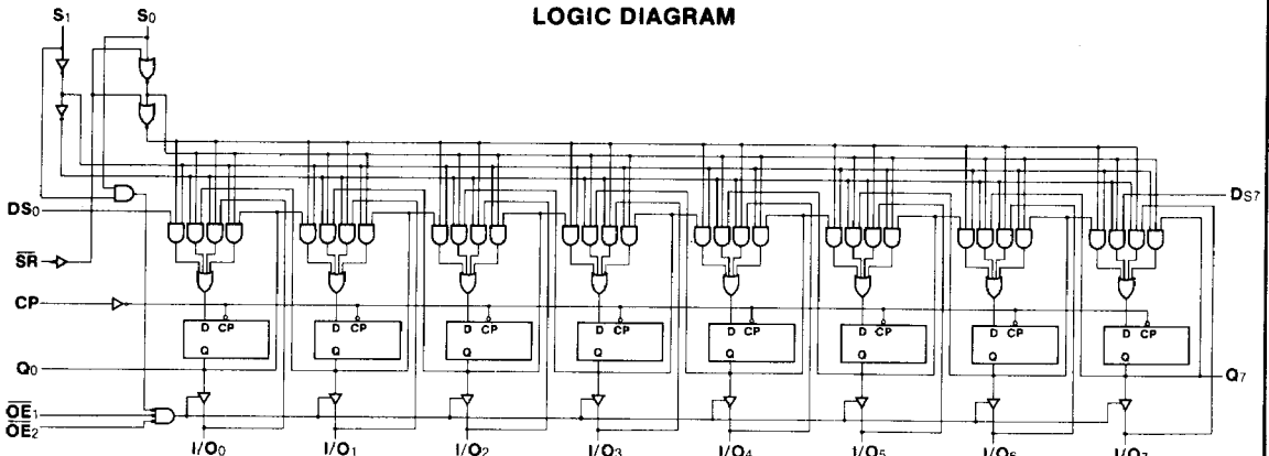
LOGIC DIAGRAM
