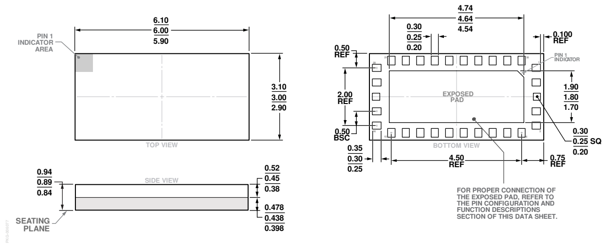
Figure 21. 30-Terminal Land Grid Array Package [LGA] (CC-30-4) Dimensions shown in millimeters
