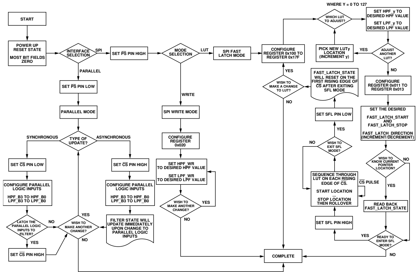
Figure 20. Programming Flowchart
