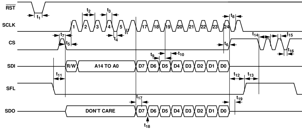
Figure 2. Timing Diagram
