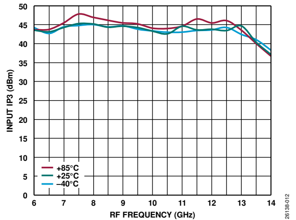
Figure 12. Input IP3 vs. RF Frequency for Various Temperatures, HPF State = 0, and LPF State = 15
