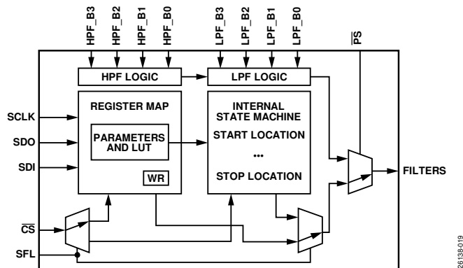
Figure 19. Simplified Interface and Logic Diagram
