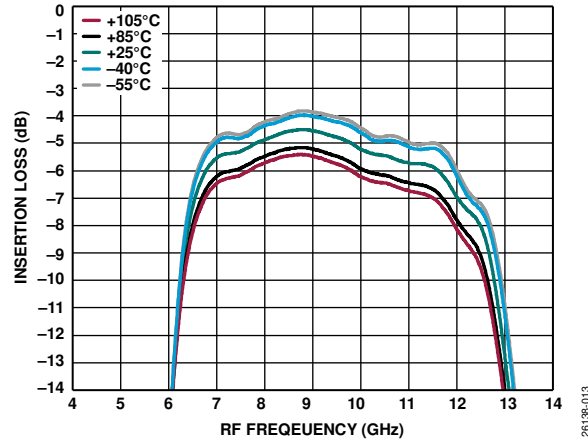
Figure 13. Insertion Loss vs. RF Frequency, Maximum Bandwidth, HPF State = 0, and LPF State = 15 for Various Temperatures
