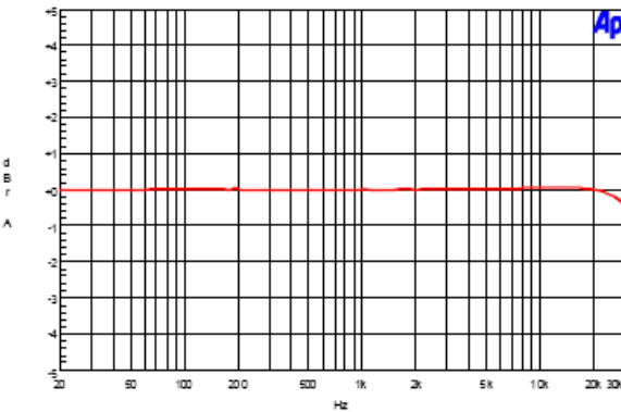
15. Frequency Response ( V_o = 1.0\text{V}_{rms} )
