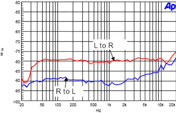
14. Crosstalk
