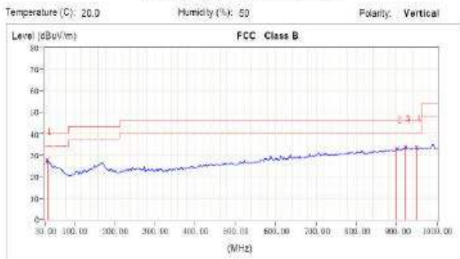
Vertical Polarization
