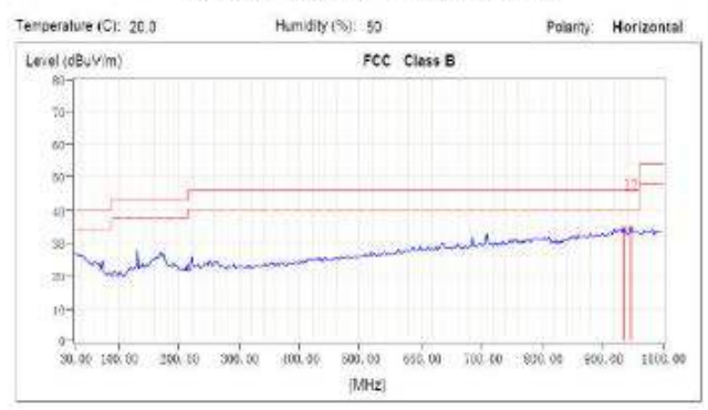
Horizontal Polarization
