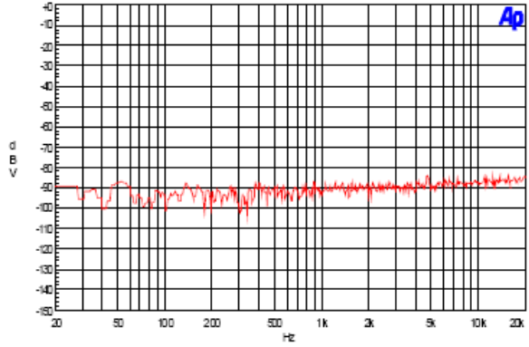
16. Noise Floor
