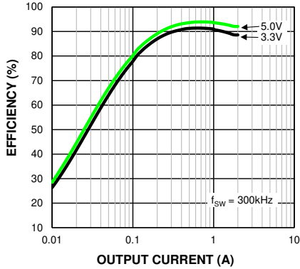
Efficiency (VIN = 12V) vs. Output Current MIC28512-2
