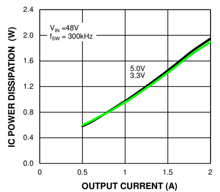
IC Power Dissipation vs. Output Current MIC28512-2
