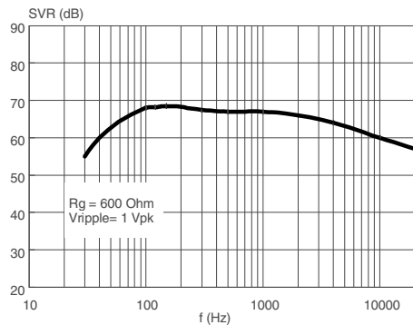
Figure 10. Supply Voltage Rejection vs. Freq.
