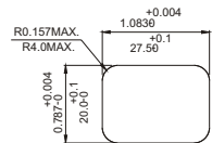
MOUNTING CUTOUT (FRONT MOUNTING)
