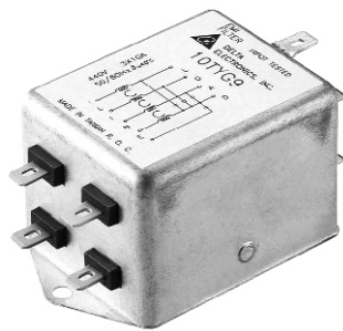
10TYG9
