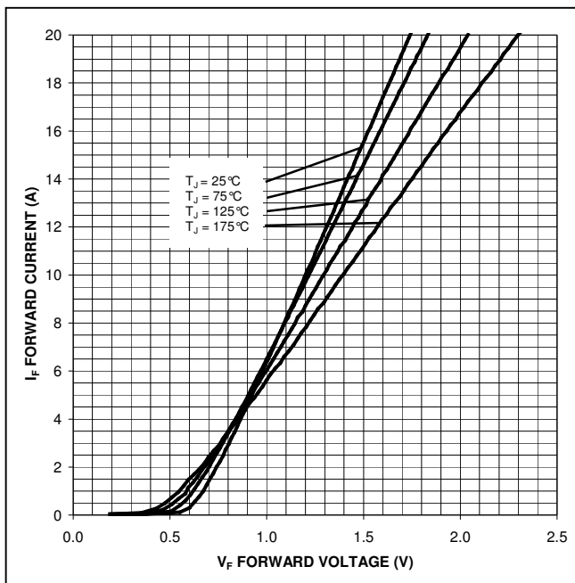
Figure 1. Forward Characteristics
