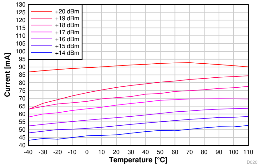
Figure 8-16. TX Current vs. Temperature (BLE 1 Mbps, 2.44 GHz, VDDS = 3.3 V)
