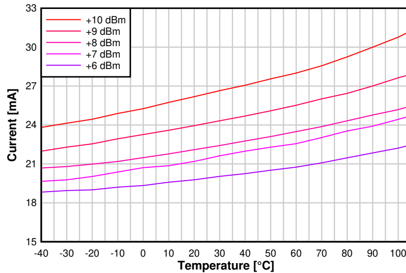
Figure 8-17. TX Current vs. Temperature (250 kbps, 2.44 GHz, +10 dBm PA)
