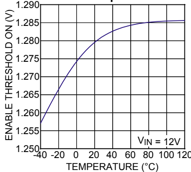
Enable Threshold ON vs. Temperature
