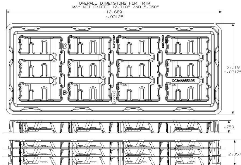
Figure 28. Through Hole Packaging Tray
