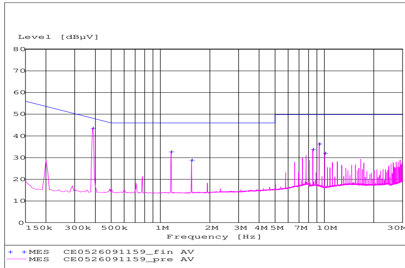
Figure 28. EMC Considerations
