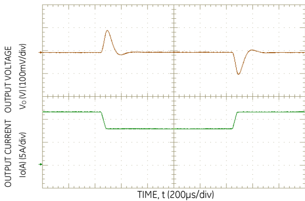
Figure 3. Transient Response to 0.1A/ \mu S Dynamic Load Change from 50% to 75% to 50% of full load ( V_{IN} = V_{IN,NOM} ).
