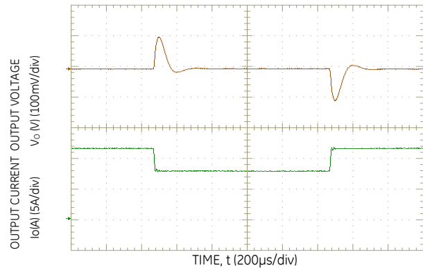
Figure 4. Transient Response to 1.0A/ \mu S Dynamic Load Change from 50% to 75% to 50% of full load ( V_{IN} = V_{IN,NOM} ).
