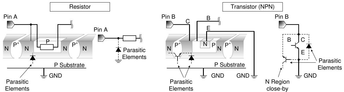
Figure 11. Example of IC Structure
