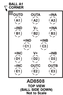
Figure 6. 14-Ball WLCSP (CB-14-1)
