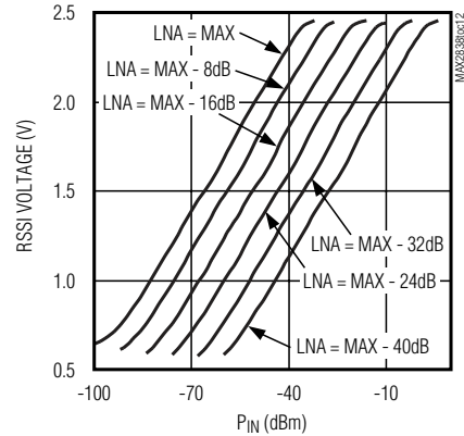
RSSI VOLTAGE vs. INPUT POWER
