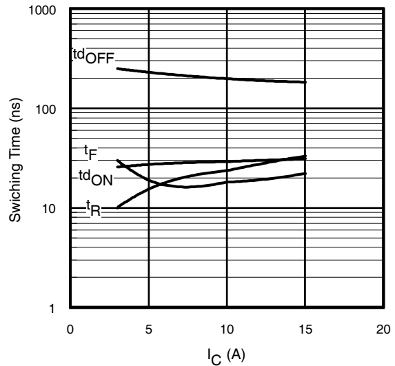
Fig. 14 - Typ. Switching Time vs. I C T J = 150°C; L=1.4mH; V CE = 400V R G = 100Ω; V GE = 15V
