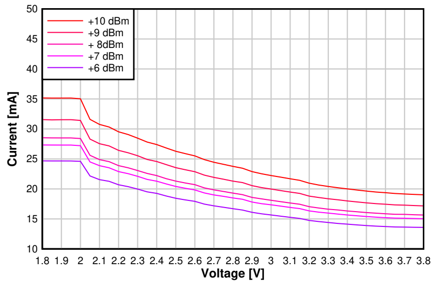
Figure 8-13. TX Current vs. Supply Voltage (VDDS) (250 kbps, 2.44 GHz, +10 dBm PA)
