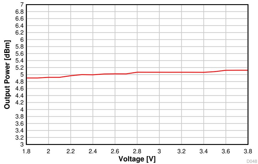
Figure 8-26. Output Power vs. Supply Voltage (VDDS) (BLE 1 Mbps, 2.44 GHz, +5 dBm)
