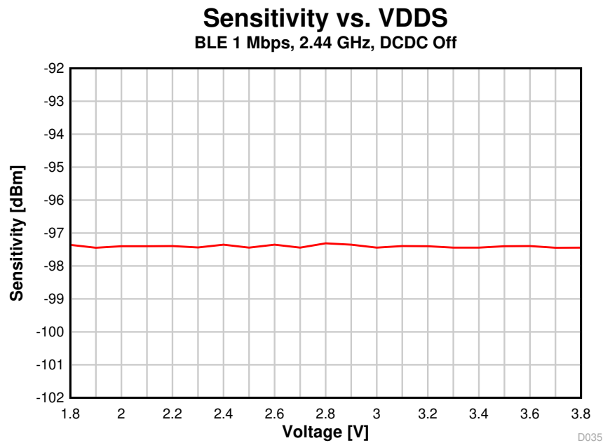
Figure 8-19. Sensitivity vs. Supply Voltage (VDDS) (BLE 1 Mbps, 2.44 GHz, DCDC Off)
