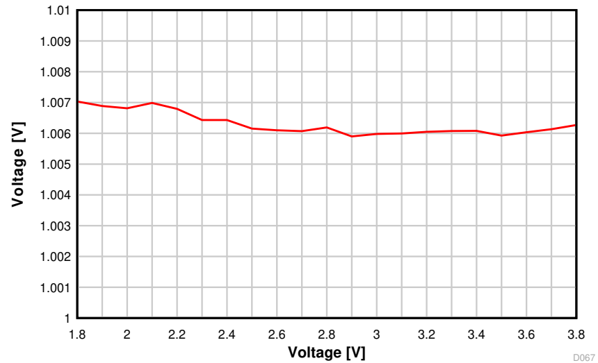
Figure 8-38. ADC Accuracy vs. Supply Voltage (VDD5)
