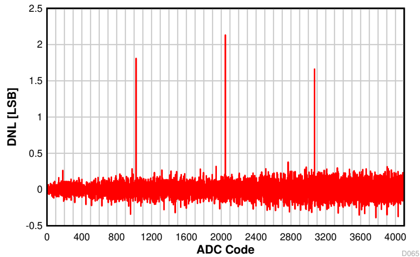
Figure 8-36. DNL vs. ADC Code
