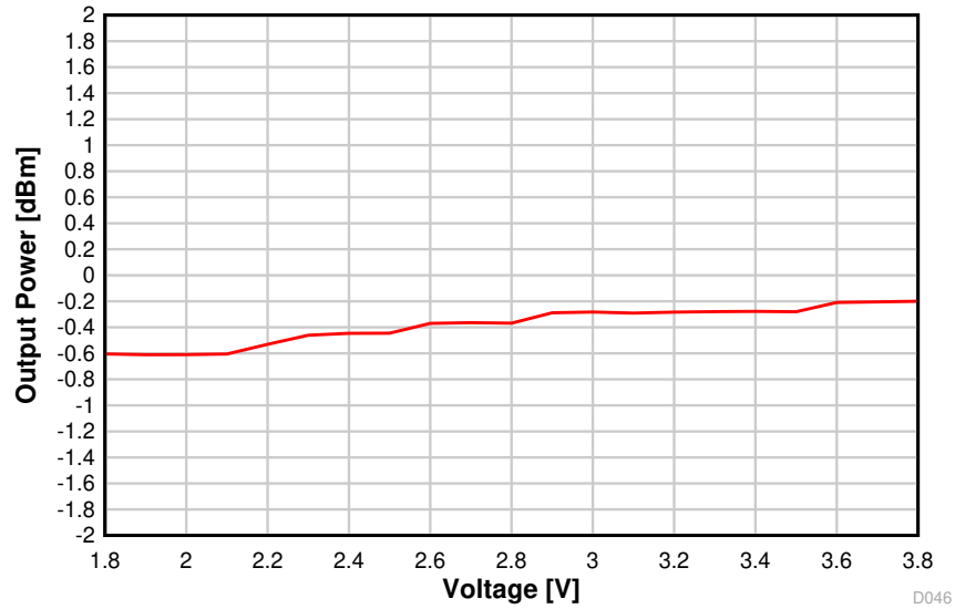
Figure 8-25. Output Power vs. Supply Voltage (VDDS) (BLE 1 Mbps, 2.44 GHz)
