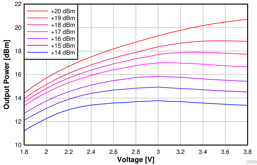
Figure 8-27. Output Power vs. Supply Voltage (VDD5) (BLE 1 Mbps, 2.44 GHz, +20 dBm PA)
