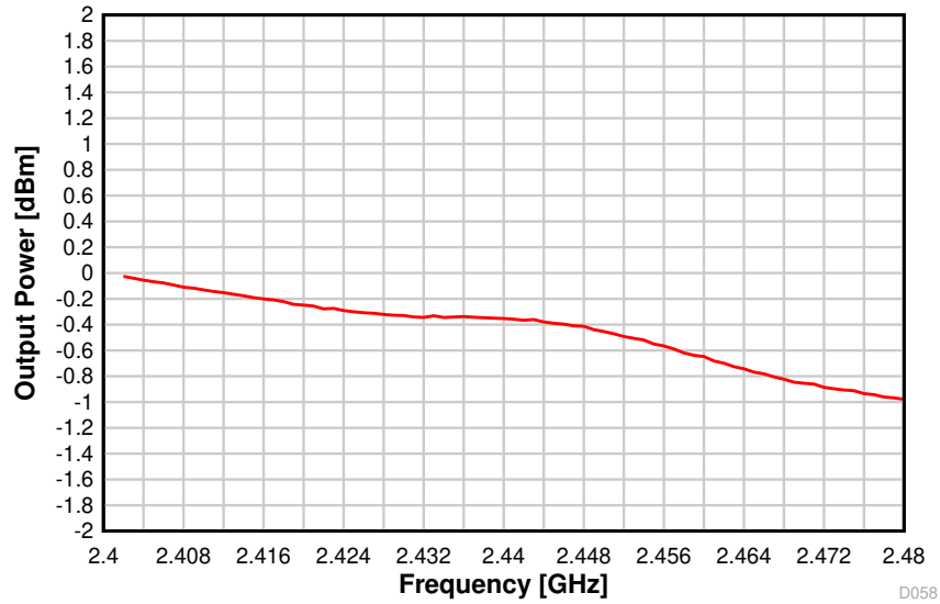
Figure 8-29. Output Power vs. Frequency (BLE 1 Mbps, 2.44 GHz)
