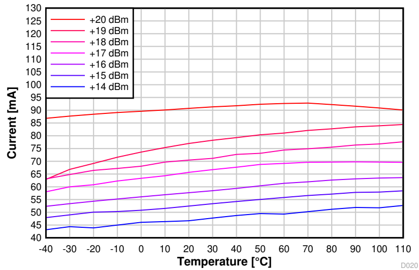
Figure 8-9. TX Current vs. Temperature (BLE 1 Mbps, 2.44 GHz, VDD5 = 3.3 V)
