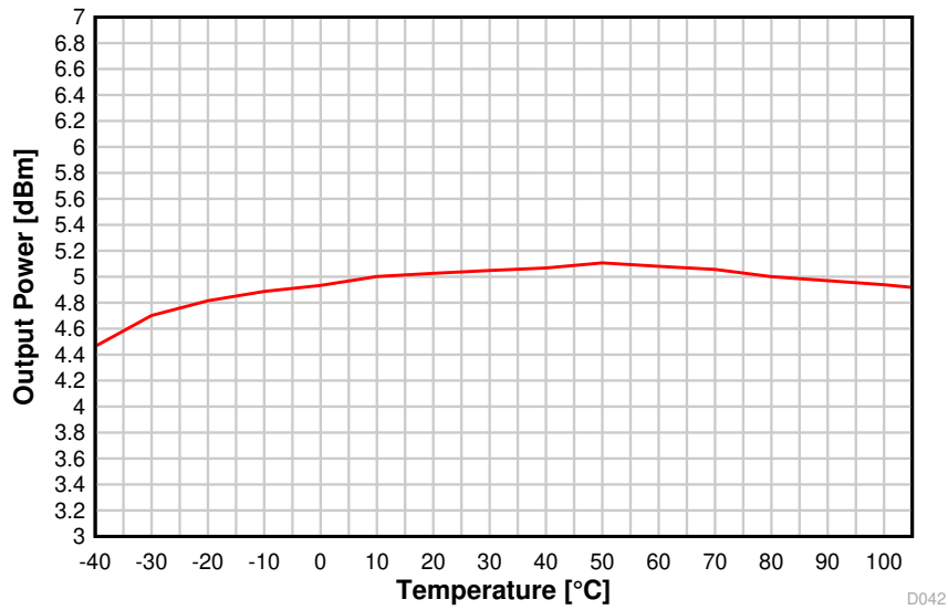
Figure 8-22. Output Power vs. Temperature (BLE 1 Mbps, 2.44 GHz, +5 dBm)
