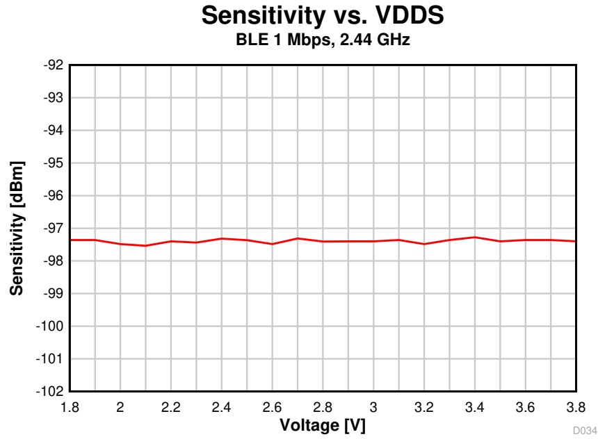
Figure 8-18. Sensitivity vs. Supply Voltage (VDDS) (BLE 1 Mbps, 2.44 GHz)
