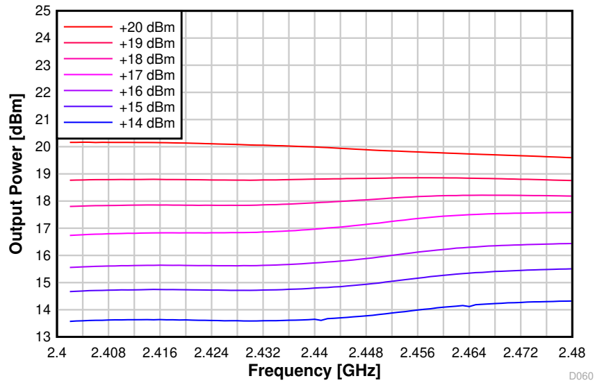
Figure 8-31. Output Power vs. Frequency (BLE 1 Mbps, 2.44 GHz, +20 dBm PA)
