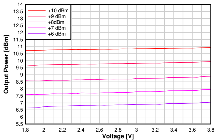
Figure 8-28. Output Power vs. Supply Voltage (VDD5) (2.44 GHz, +10 dBm PA)
