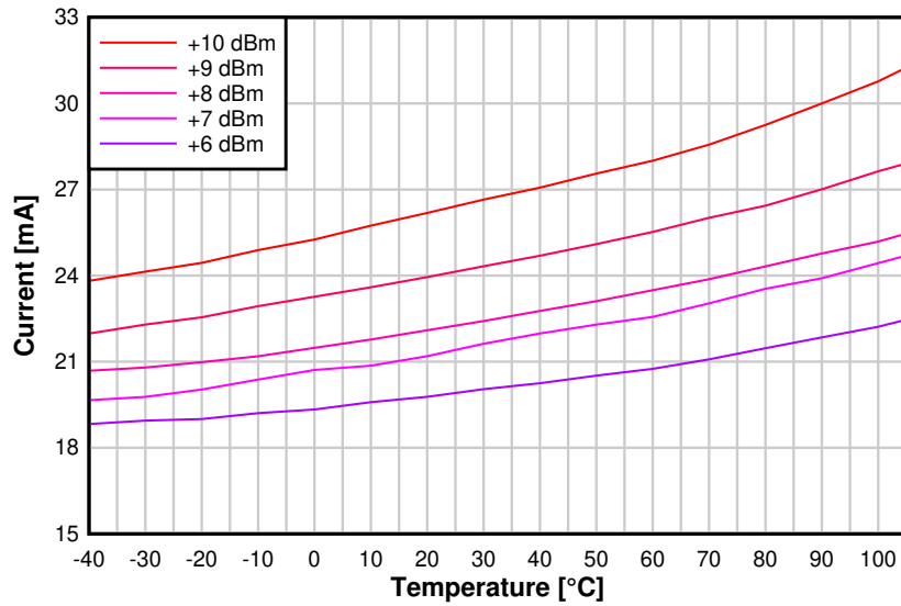
Figure 8-10. TX Current vs. Temperature (250 kbps, 2.44 GHz, +10 dBm PA)
