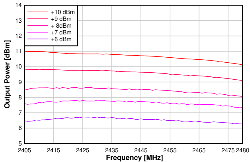
Figure 8-32. Output Power vs. Frequency (250 kbps, +10 dBm PA)
