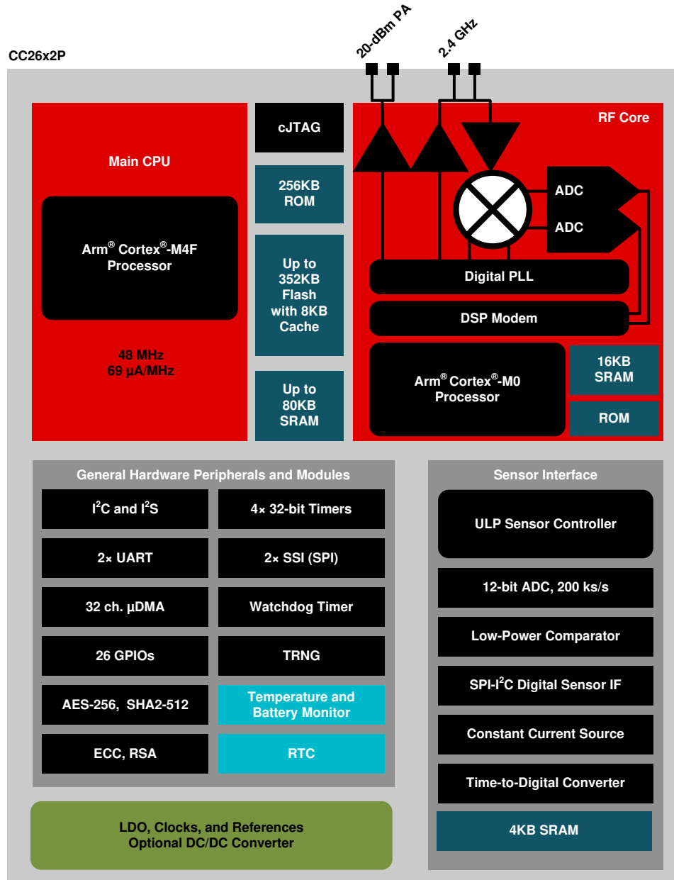
Figure 4-1. CC2652P Block Diagram
