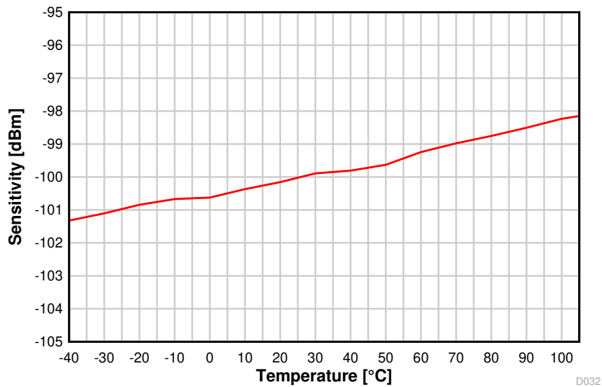
Figure 8-17. Sensitivity vs. Temperature (250 kbps, 2.44 GHz)
