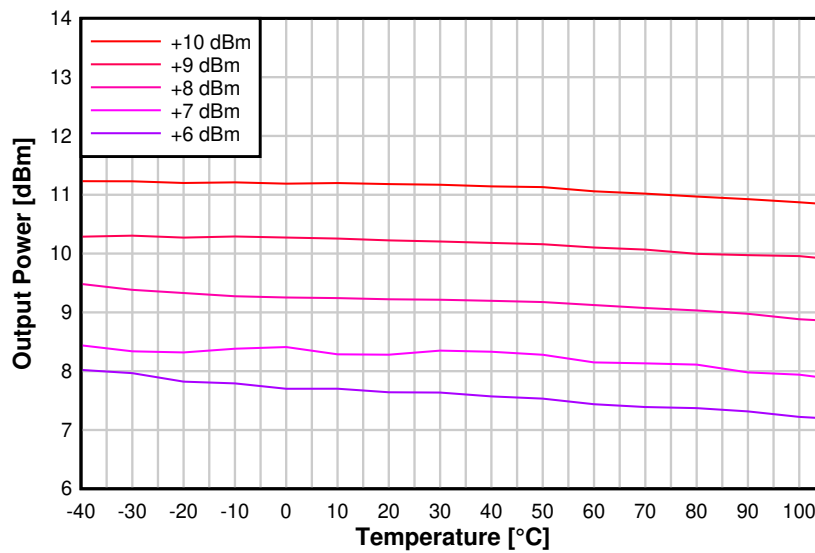
Figure 8-24. Output Power vs. Temperature (2.44 GHz, +10 dBm PA)
