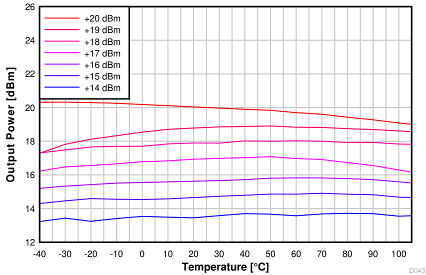
Figure 8-23. Output Power vs. Temperature (BLE 1 Mbps, 2.44 GHz, +20 dBm PA)
