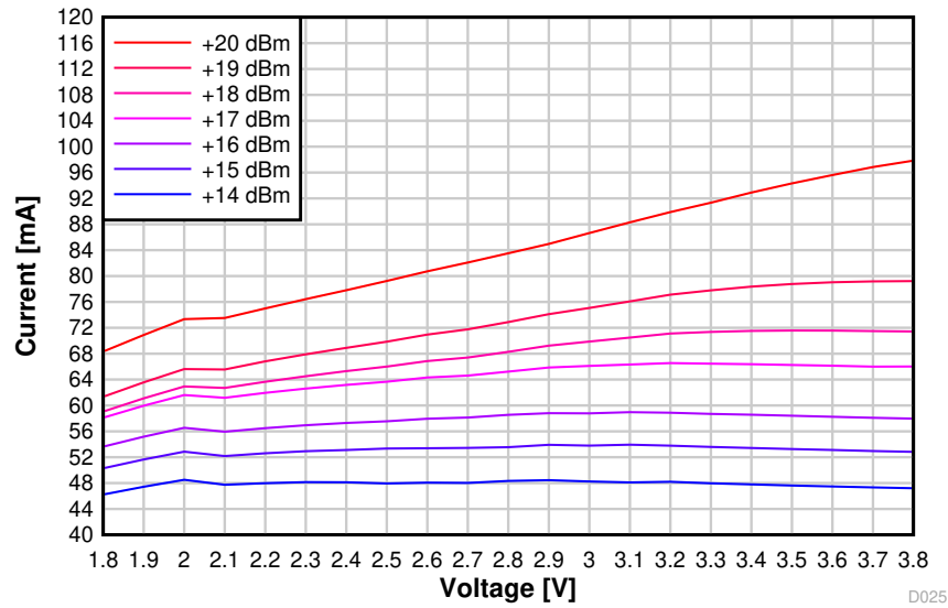
Figure 8-12. TX Current vs. Supply Voltage (VDDS) (BLE 1 Mbps, 2.44 GHz, +20 dBm PA)
