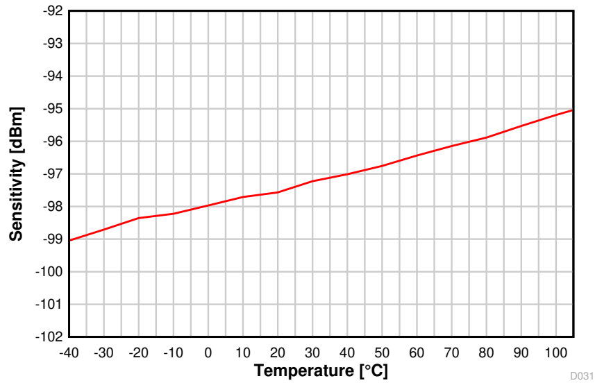
Figure 8-16. Sensitivity vs. Temperature (BLE 1 Mbps, 2.44 GHz)
