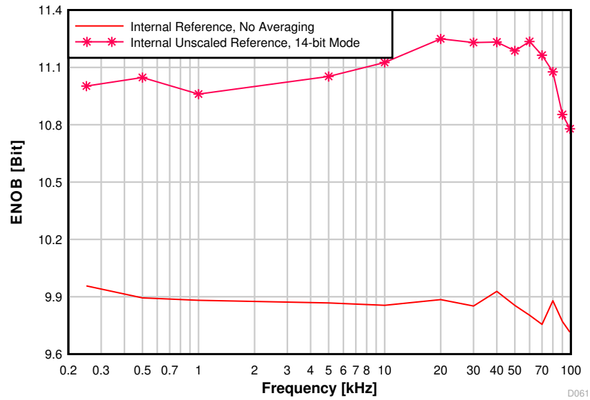
Figure 8-33. ENOB vs. Input Frequency
