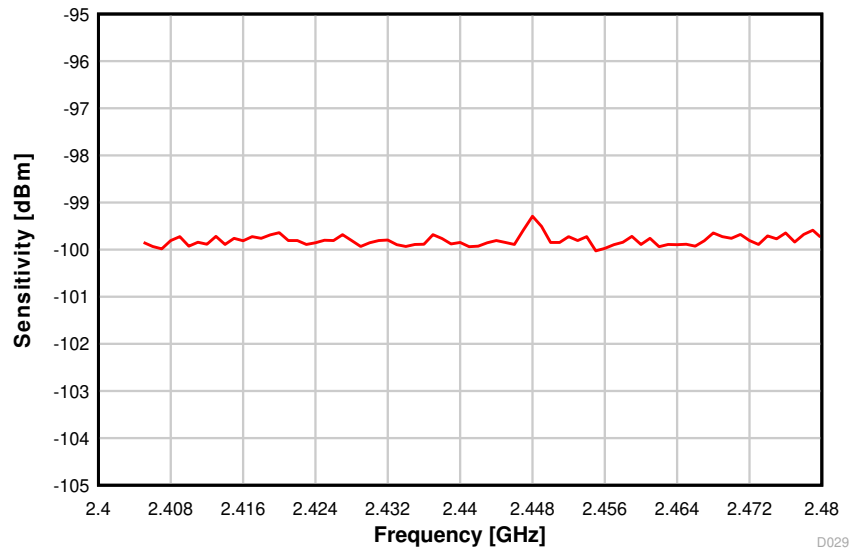
Figure 8-15. Sensitivity vs. Frequency (250 kbps, 2.44 GHz)
