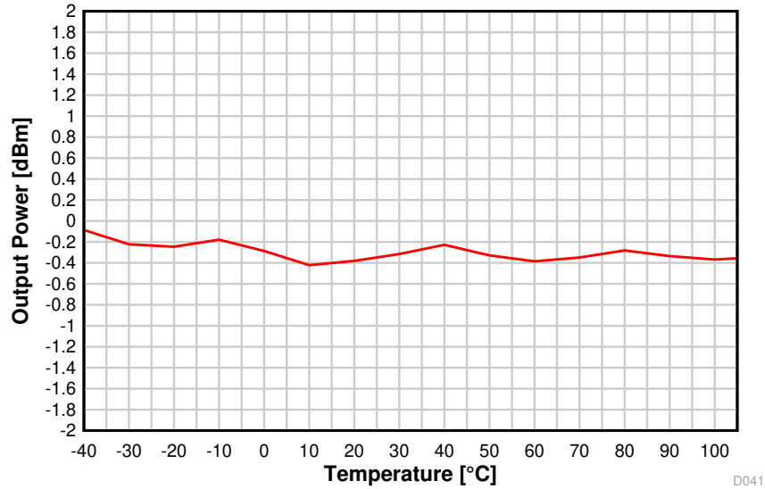
Figure 8-21. Output Power vs. Temperature (BLE 1 Mbps, 2.44 GHz)
