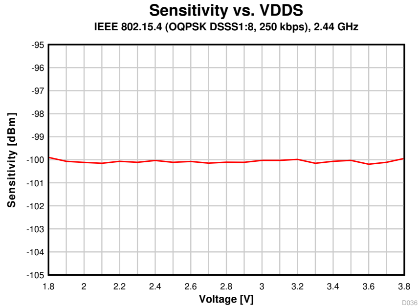
Figure 8-20. Sensitivity vs. Supply Voltage (VDDS) (250 kbps, 2.44 GHz)
