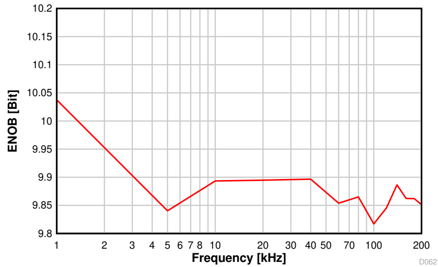
Figure 8-34. ENOB vs. Sampling Frequency
