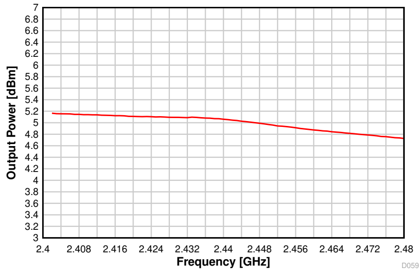
Figure 8-30. Output Power vs. Frequency (BLE 1 Mbps, 2.44 GHz, +5 dBm)
