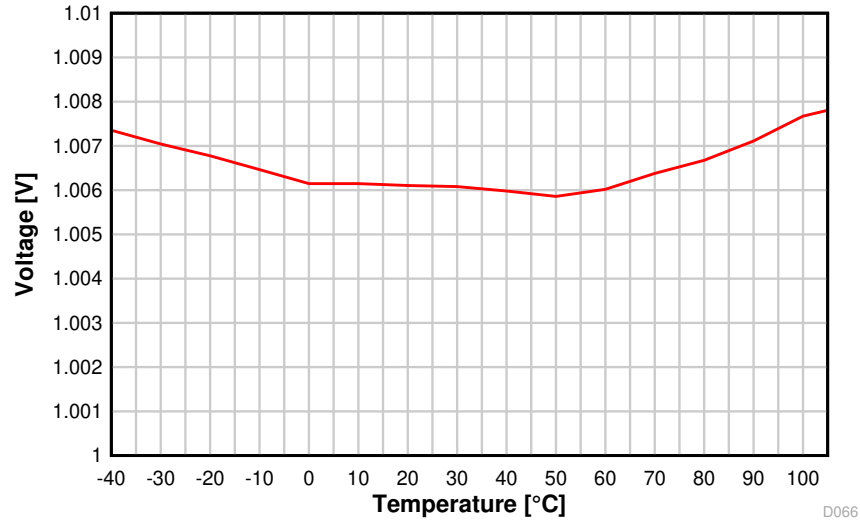
Figure 8-37. ADC Accuracy vs. Temperature
