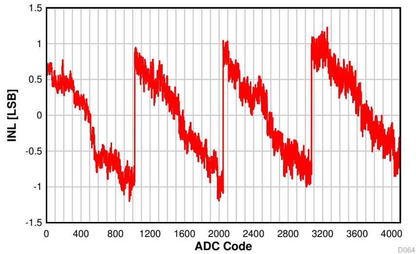
Figure 8-35. INL vs. ADC Code
