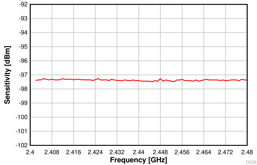
Figure 8-14. Sensitivity vs. Frequency (BLE 1 Mbps, 2.44 GHz)
