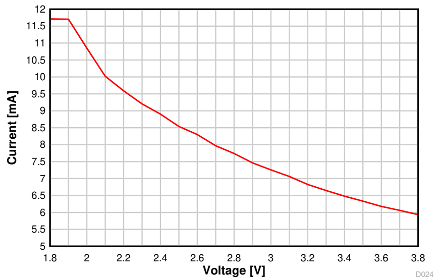
Figure 8-11. TX Current vs. Supply Voltage (VDD5) (BLE 1 Mbps, 2.44 GHz)
