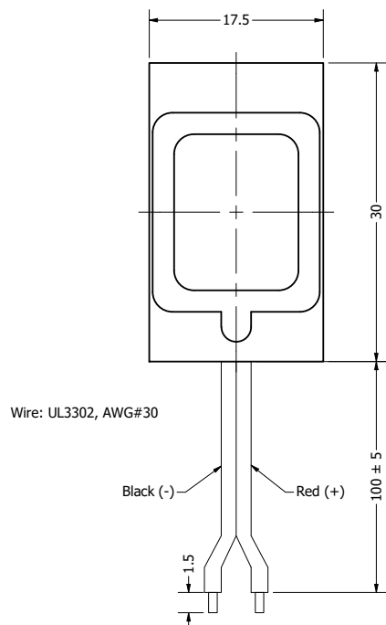
Top View
