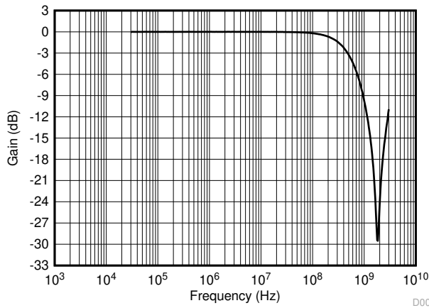
Figure 6-9. Insertion Loss
