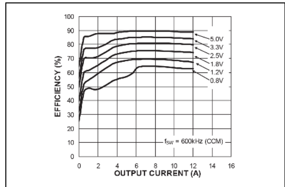
FIGURE 2-17: Efficiency ( V_{IN} = 24V ) vs. Output Current (MIC2101).
