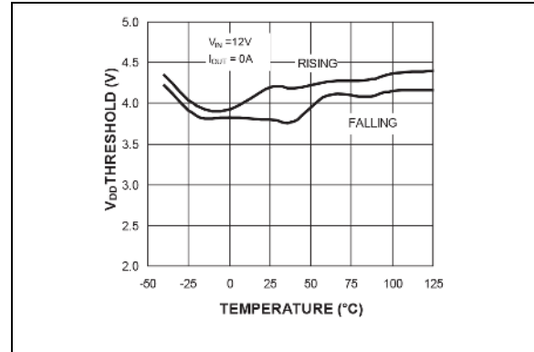
FIGURE 2-52: V_{DD} UVLO Threshold vs. Temperature.
