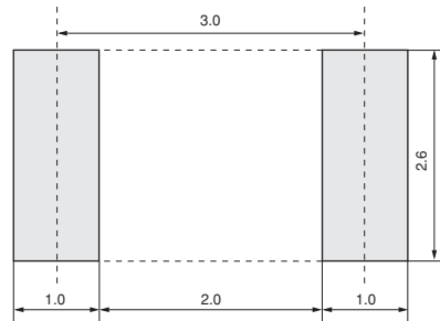
CDESCB Series
