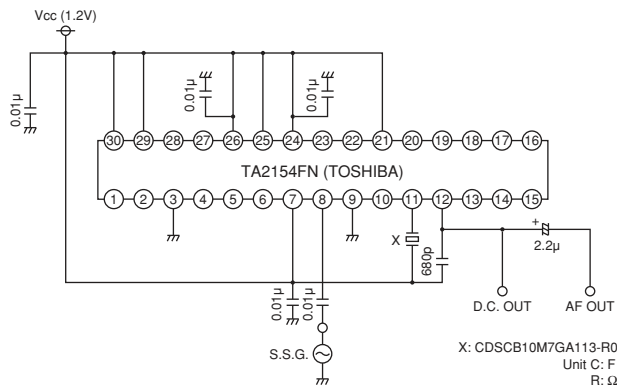
CDSCB10M7GA113-R0
