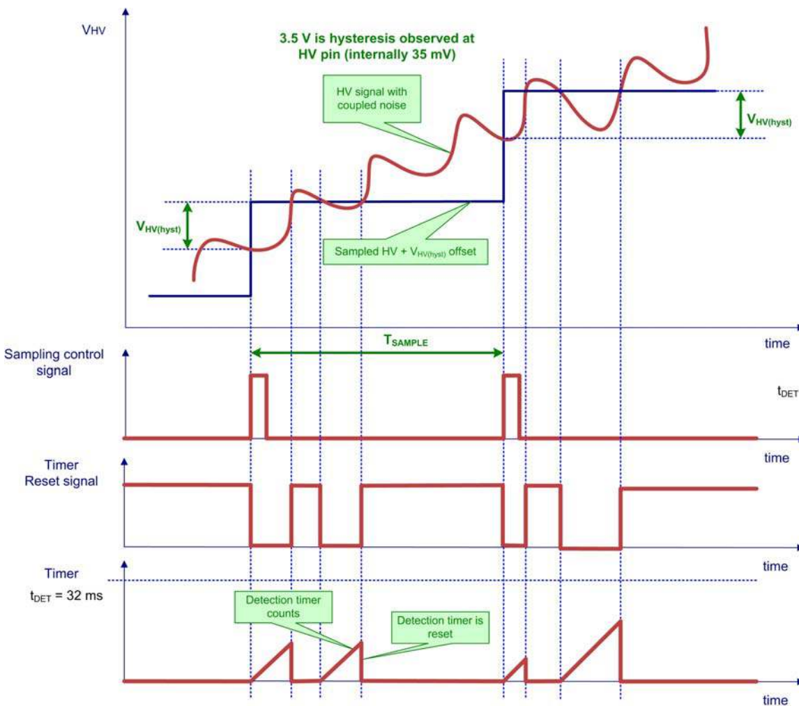
Figure 52. The ac Line Unplug Detector Timing Diagram Detail with Noise Effects
