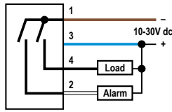
Alarm Hookup
