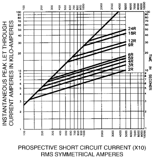
4.8 kV Peak let-through curves for JCL_R and JCL-A_R (2R-24R @25°C)
