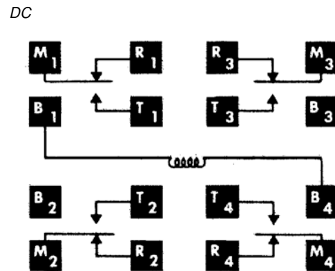
GP Series Terminal Diagram
