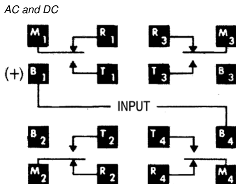
TR Series Terminal Diagram
