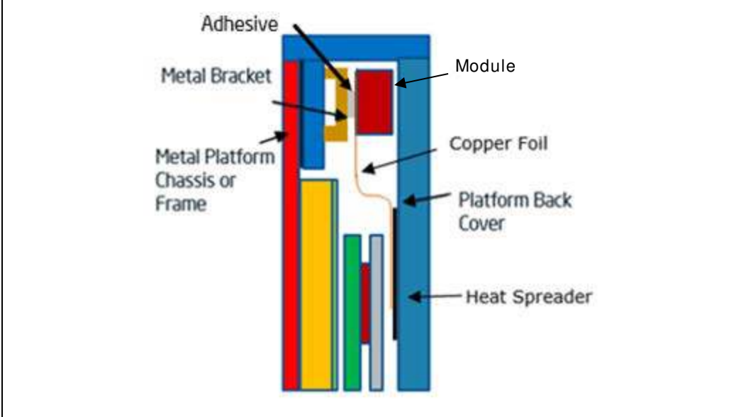
Figure 7-13. Module Thermal Solution Rear Cover Mount
