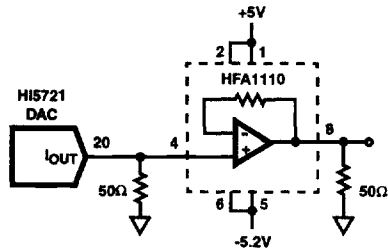
FIGURE 23. HIGH SPEED CURRENT TO VOLTAGE CONVERSION
