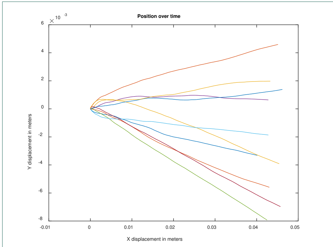
Fig 14. XY displacement over a 5 second interval (10 runs) for a calibrated accelerometer
