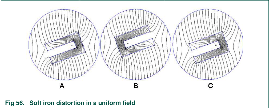
Fig 56. Soft iron distortion in a uniform field Soft iron, you say? What’s that? Think steel. Think EMI shields, screws and battery contacts. To illustrate the point, we performed a finite elements simulation of a U-shaped piece of steel sitting in a uniform magnetic field. Fig 56A shows how the magnetic field (which would otherwise be shown as vertical lines) is distorted by the presence of our “U-bar”. Steel provides a “lower resistance” path to the magnetic field than does the surrounding air. So it is natural for the field to be diverted. Fig 56B takes that same U-bar and rotates it exactly 180 degrees in the same ambient field. You can see similarities in the field distortion. We can see just how similar Fig 56A and Fig 56B are by taking Fig 56B and flipping it, first about one axis and then the other, to obtain Fig 56C, which is identical in form to Fig 56A.
