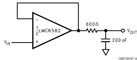
FIGURE 7. Resistive Isolation of a 350 pF Capacitive Load
