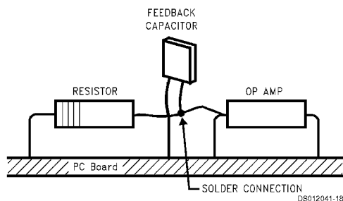
FIGURE 13. Air Wiring
