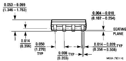
8-Pin Small Outline Package Order Number LMC6582AIM or LMC6582BIM NS Package Number M08A
