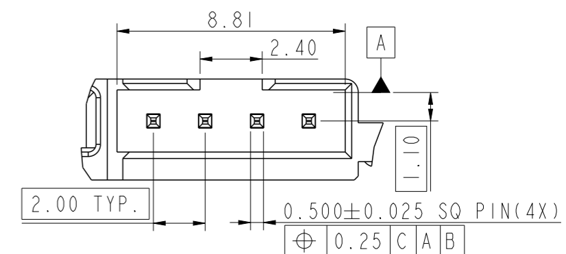
DETAIL A SCALE 5.000
