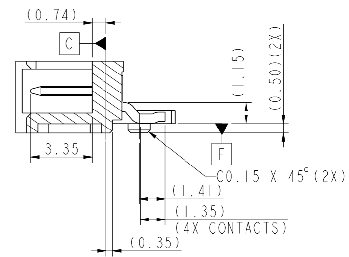
SECTION C-C SCALE 5.000
