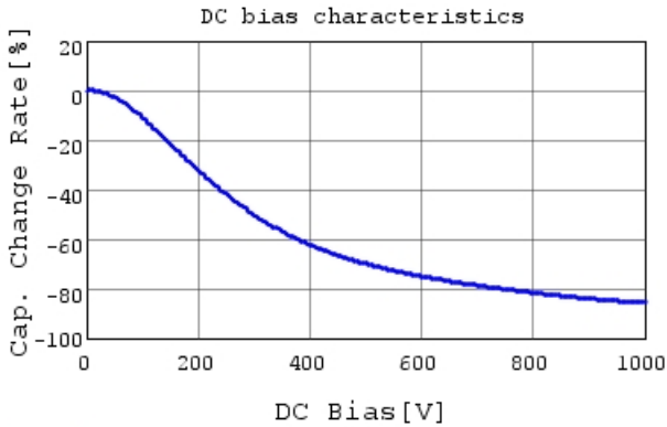
RDER73A104K5B1H03B C-DC bias capchange, 25.0
