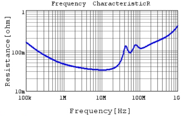
RDER73A104K5B1H03B R DCOV, 25degC
