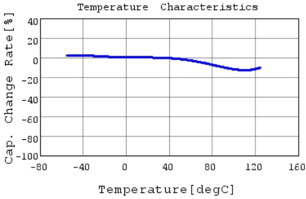
RDER73A104K5B1H03B C-Temp. capchange, DCOV,
