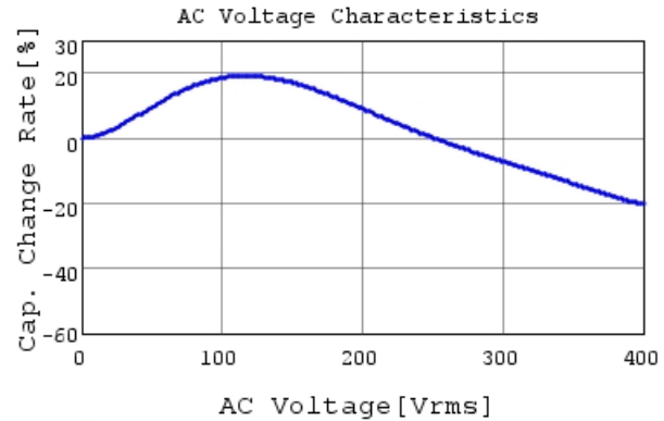
RDER73A104K5B1H03B C-AC Voltage capchange, I
