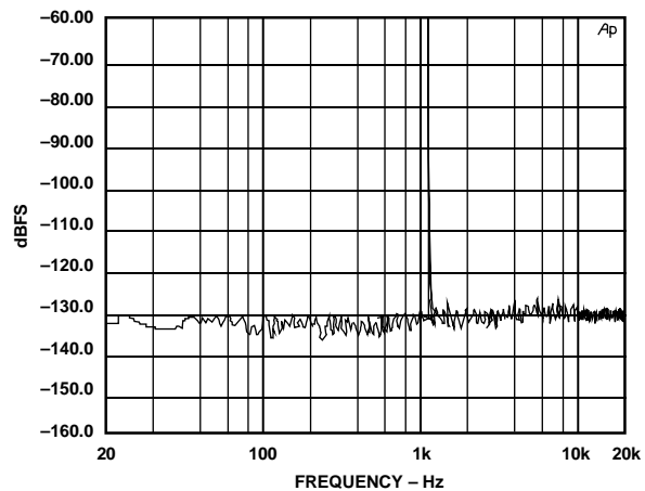
Figure 14b. AD1891—Dynamic Range from 20 Hz to 20 kHz, -60 dBFS, 48 kHz Input Sample Frequency, 44.1 kHz Output Sample Frequency, 16k-Point FFT, BH4 Window
