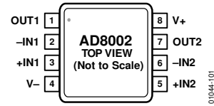
Figure 5. 8-Lead MSOP
