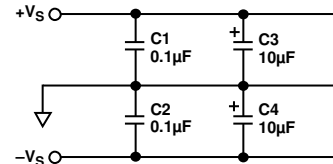
Figure 58. Supply Bypassing
