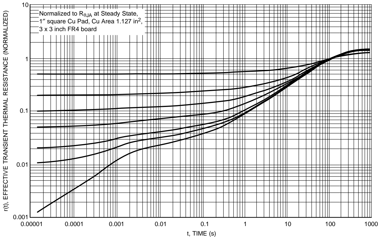
Figure 14. Thermal Response
