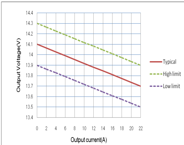
Figure 9: Output voltage vs. Output current @ Vin=48V. Drog function.
