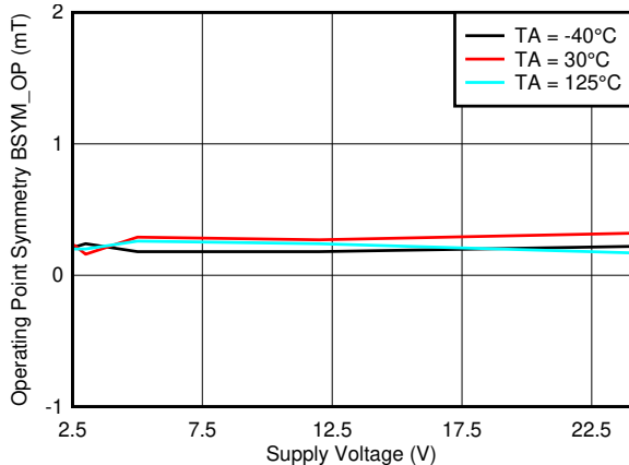
Figure 7-29. B_{SYM\_OP(ZY)} vs. V_{CC}
