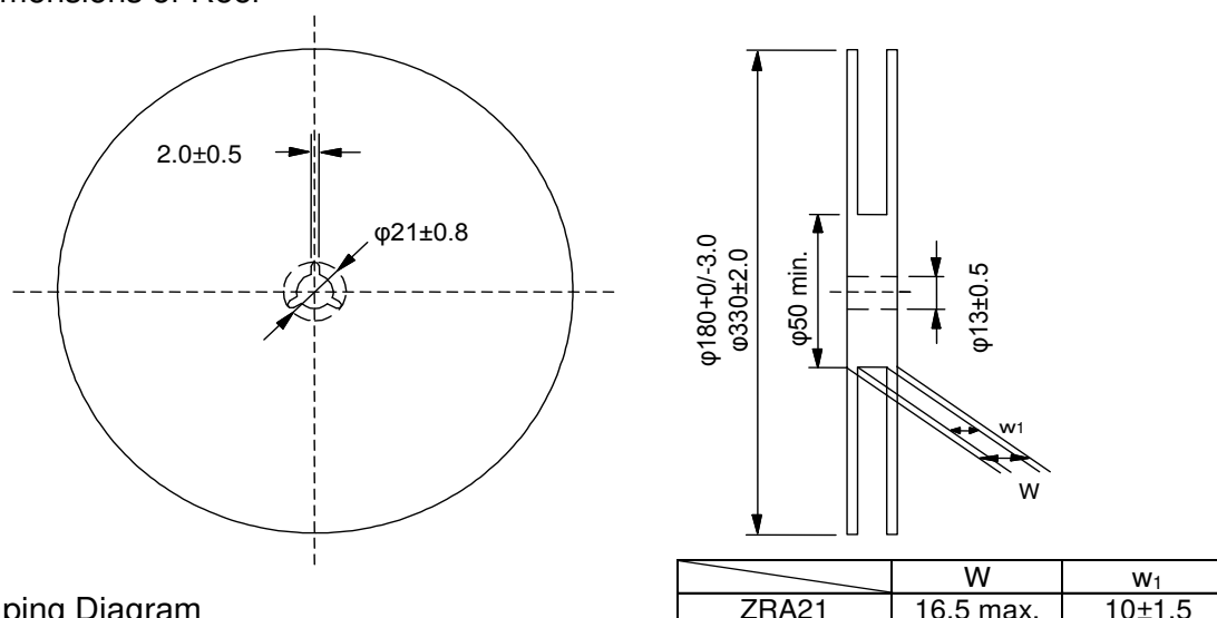
Fig.2 Dimensions of Reel
