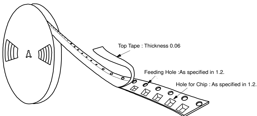
Fig.3 Taping Diagram
