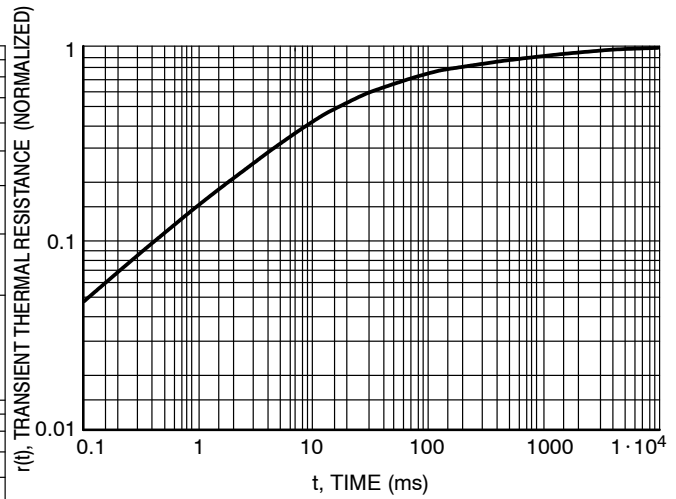
Figure 4. Thermal Response
