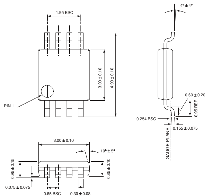
MSOP-8
