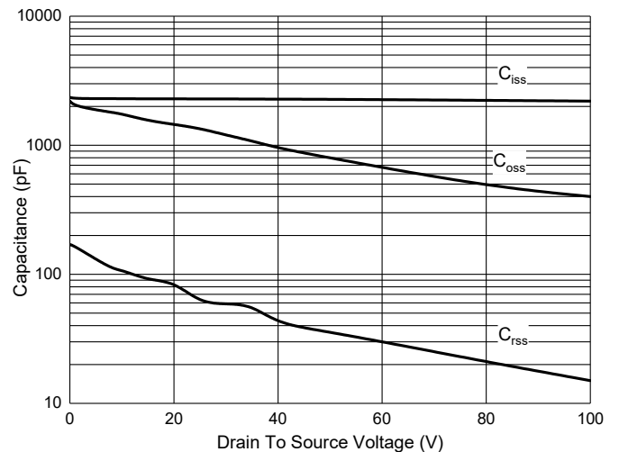
Fig. 6 - Capacitance Characteristics
